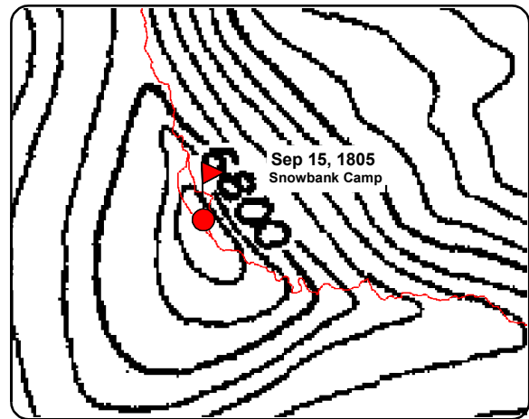
Figure 1. Precision GPS data plotted on a USGS topographic map. The map has topographic distortion which puts the ridge line too far south and west.
