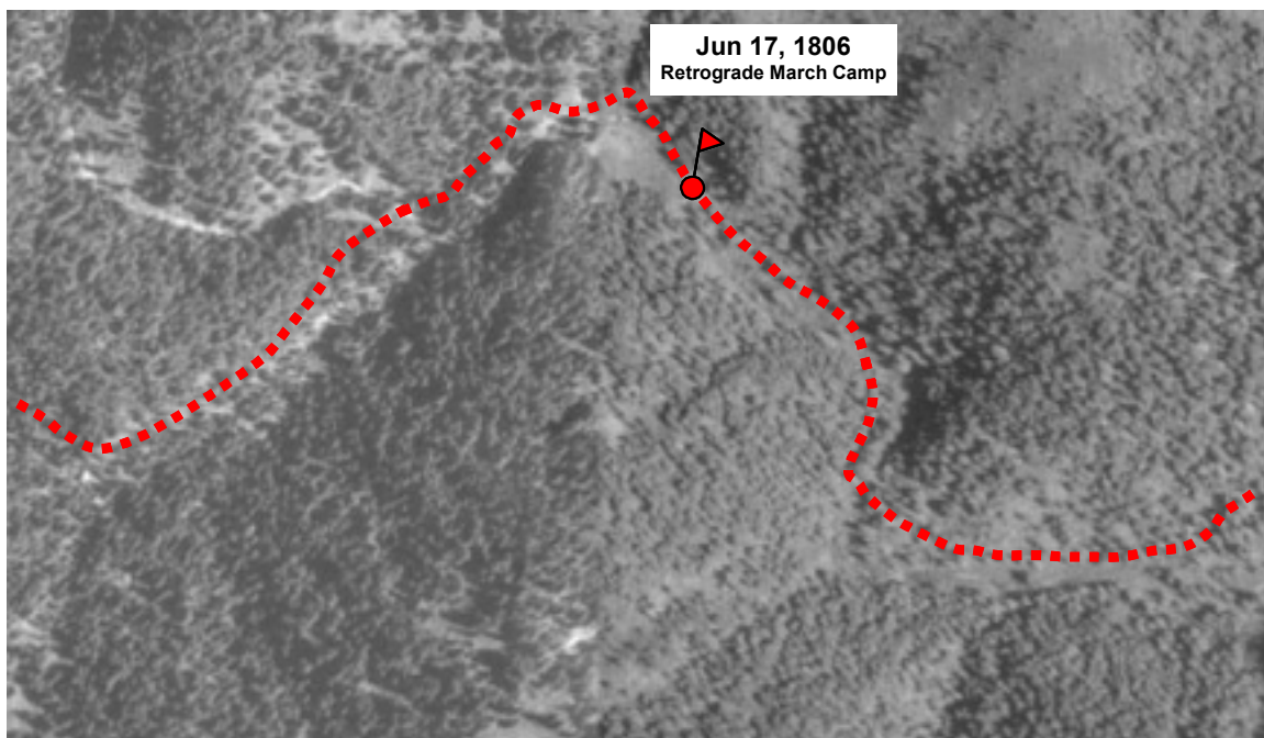
Figure 4. Aerial photo of exact area covered by the topo map above.
