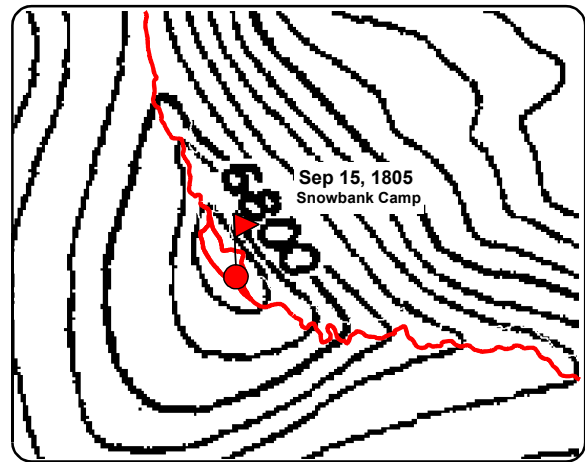
Figure 2. Trail plot distorted to match the topographic distortion of the map at Snowbank Camp.
