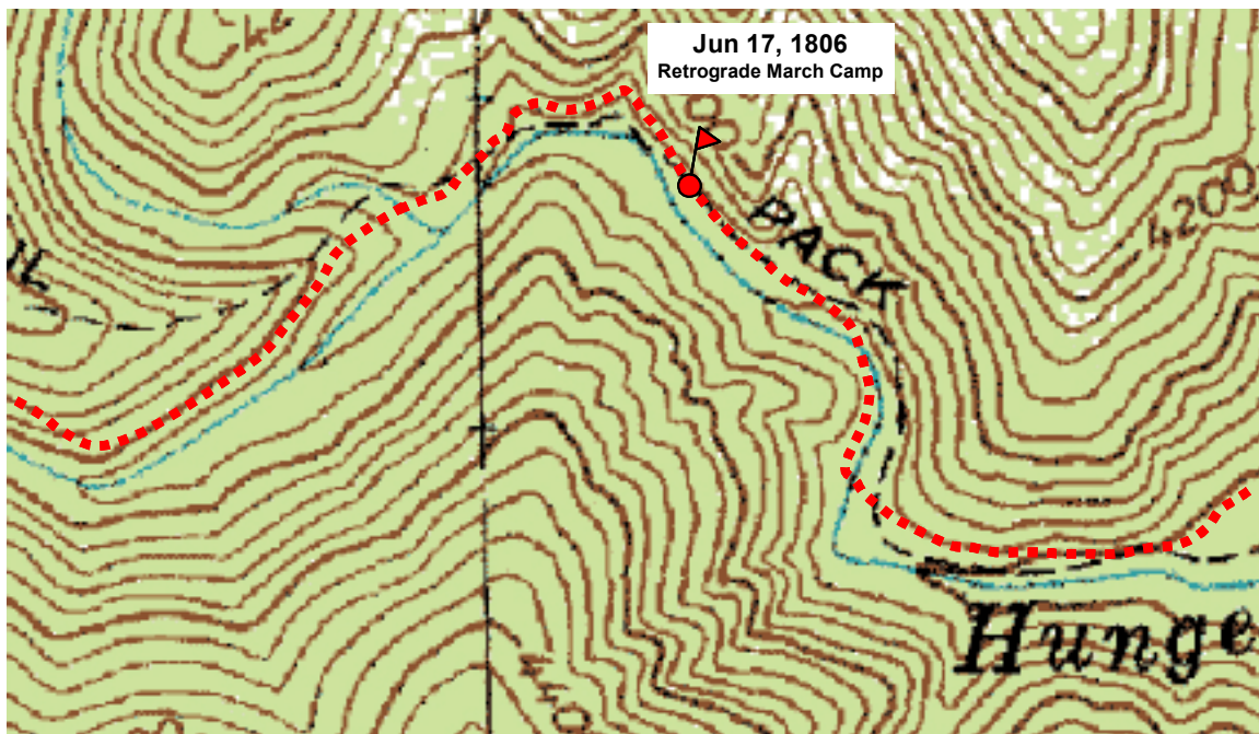
Figure 3. Hungry Creek at the mouth of Obia Creek. This map and the aerial photo below are exactly aligned to show the trail and campsite relative to a topo map and an aerial photo. Refer to maps LCT-Survey-19 and LCT-Survey-20 for a larger area of coverage.
